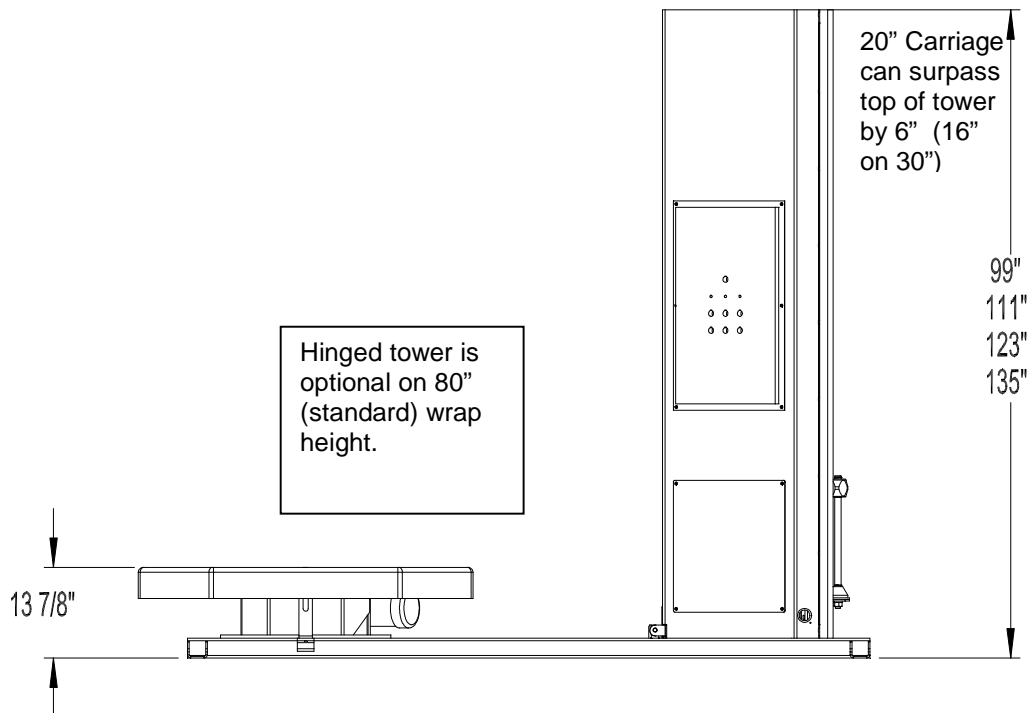
MODEL SMH-HVY – 8,000 lb. CAPACITY EXTRA HEAVY-DUTY BASE, HIGH-PROFILE SMART™ SERIES STRETCH WRAPPER (WITH NO-THREAD® POWERED PRE-STRETCH CARRIAGE)
