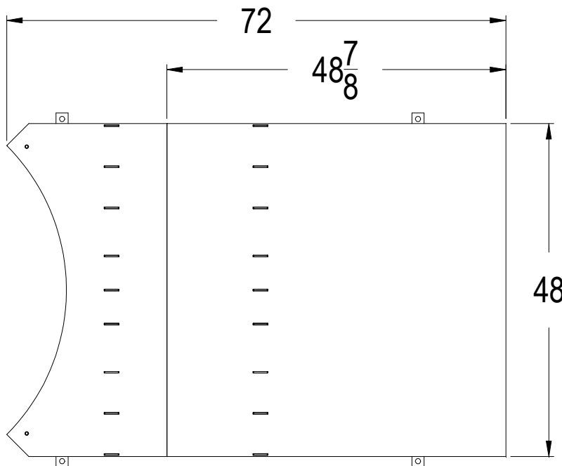
MODEL SML-150 – 58" DIAMETER 4,000 lb. CAPACITY OCTAGONAL BASE, LOW-PROFILE SMART SERIES STRETCH WRAPPER (WITH NO-THREAD® POWERED PRE-STRETCH CARRIAGE) FINISHED VIEW WITH THE RAMP
