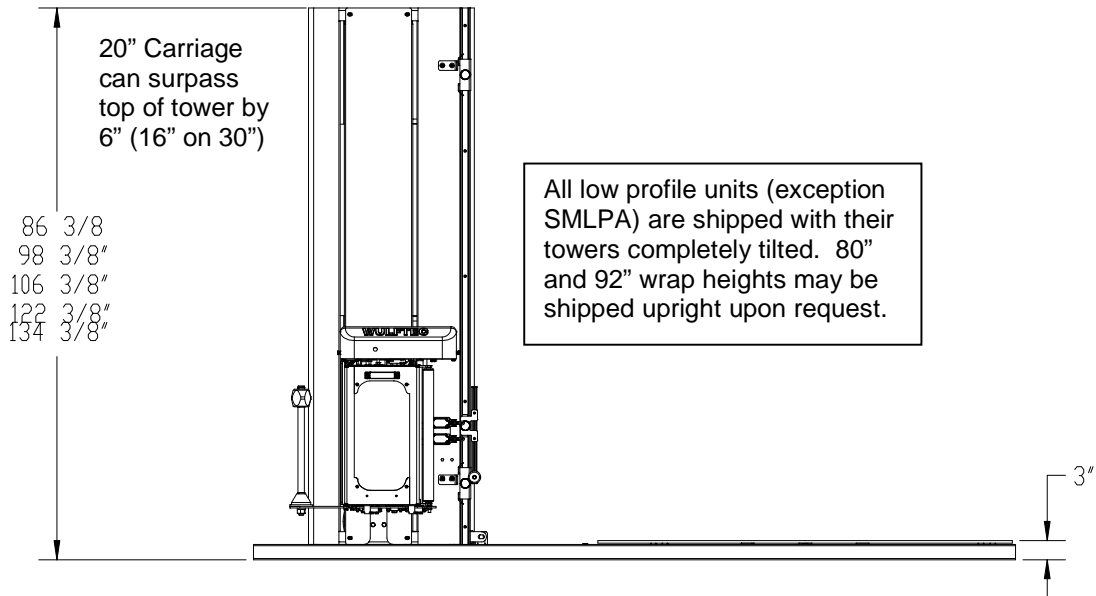
MODEL SML-200 – 65" DIAMETER 5,000 lb. CAPACITY STANDARD TURNTABLE, LOW-PROFILE SMART™ SERIES STRETCH WRAPPER (WITH NO-THREAD® POWERED PRE-STRETCH CARRIAGE)
