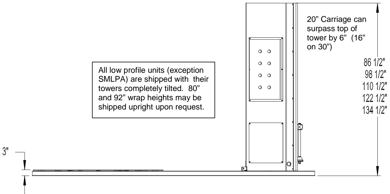
MODEL SML-EXT – 65" DIAMETER 5,000 lb. CAPACITY STANDARD TURNTABLE WITH 2' EXTENSION BASE, LOW-PROFILE SMART™ SERIES STRETCH WRAPPER (WITH NO-THREAD® POWERED PRE-STRETCH CARRIAGE)
