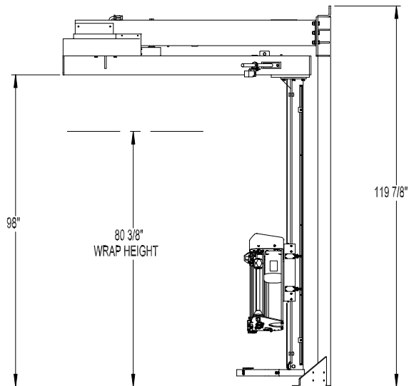
MODEL WRT-100 SEMI-AUTOMATIC COLUMN-MOUNTED ROTARY ARM (WITH NO-THREAD ® POWERED PRE-STRETCH CARRIAGE)
