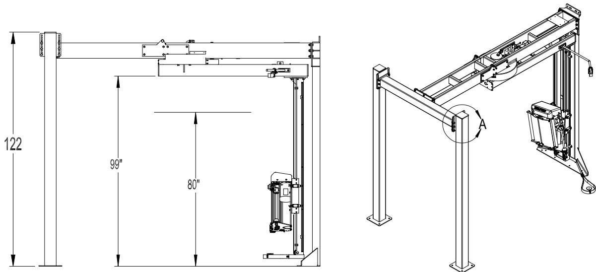
MODEL WRT-175 SEMI-AUTOMATIC SELF-SUPPORTING 3-LEGGED ROTARY ARM (WITH NO-THREAD® POWERED PRE-STRETCH CARRIAGE)
