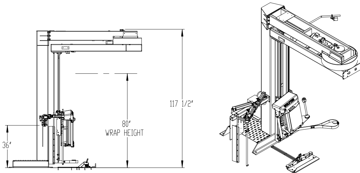
MODEL WRTA-150 NON-CONVEYORIZED AUTOMATIC FLOOR-MOUNTED ROTARY ARM (WITH NO-THREAD® POWERED PRE-STRETCH CARRIAGE)
